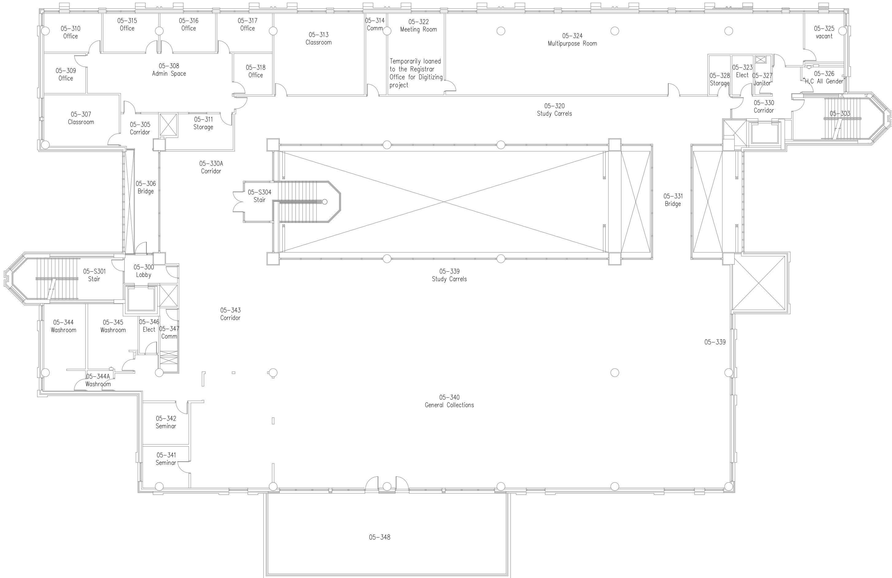
LIBRARY — THIRD FLOOR PLAN
