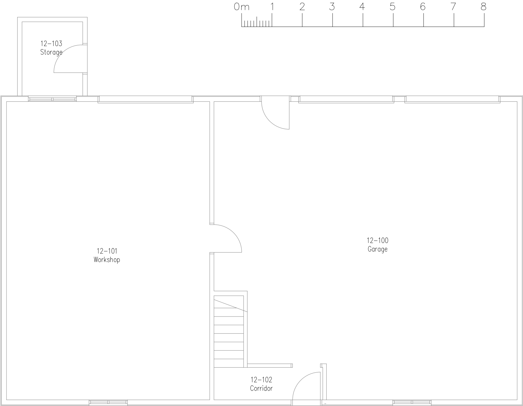
MAINTENANCE BUILDING MAIN FLOOR
